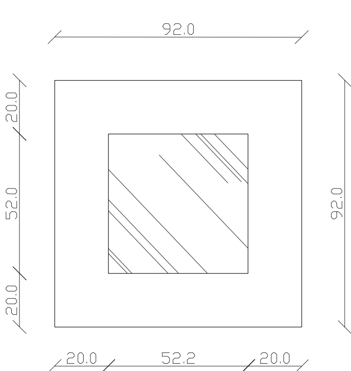
SPECCHIO VISTA FRONTALE / front view mirror
