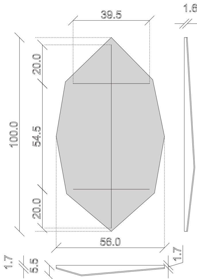
SPECCHIO VISTA RETRO / rear view mirror
