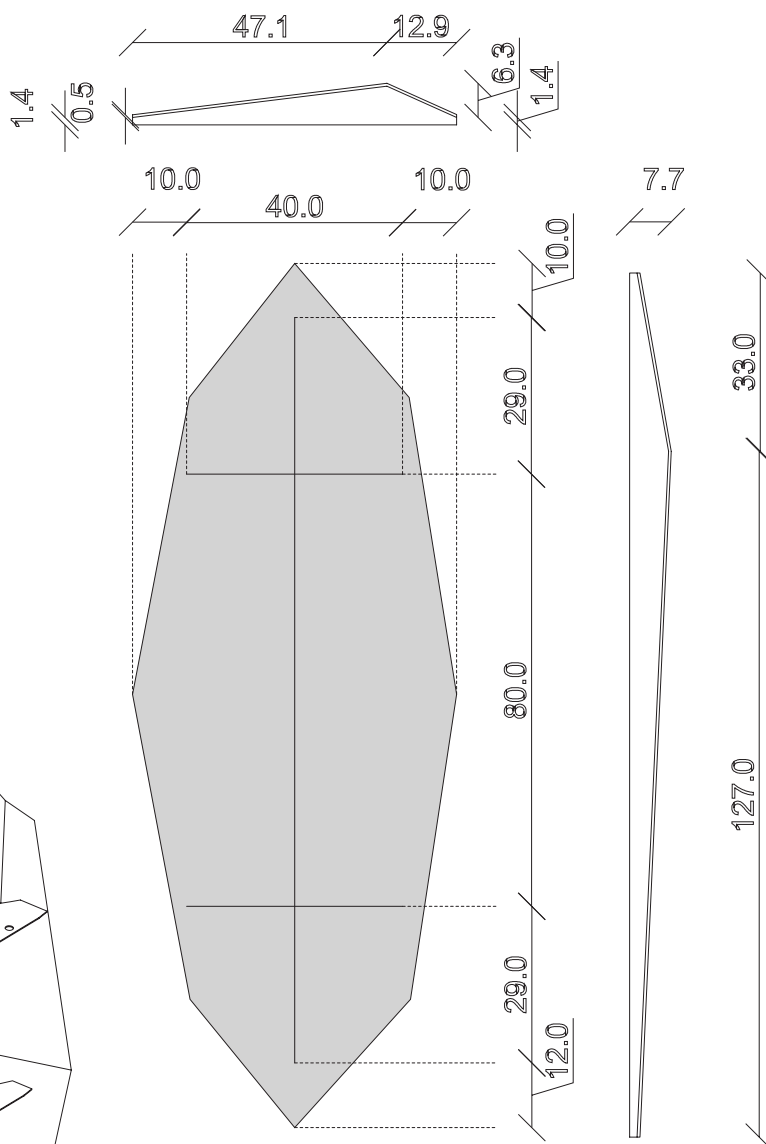
SPECCHIO VISTA RETRO / rear view mirror
