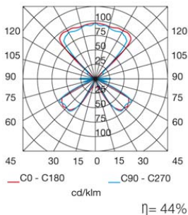
E-27 100W
