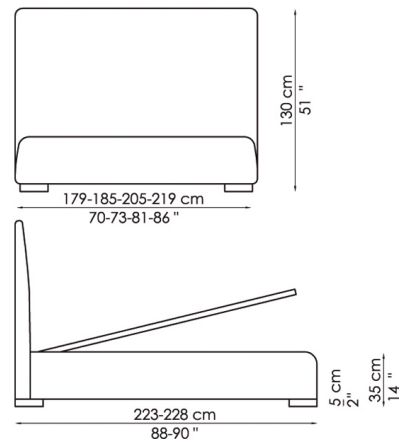
Bloom alto contenitore with storage
