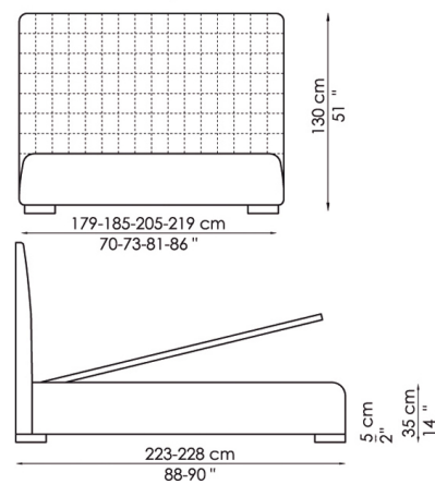
Bloom ego contenitore with storage
