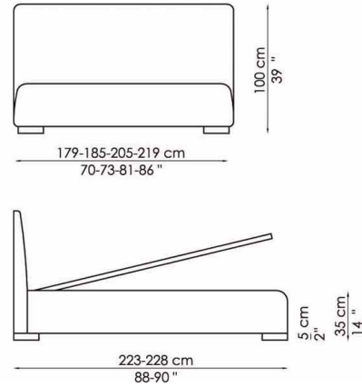
Bloom contenitore with storage
