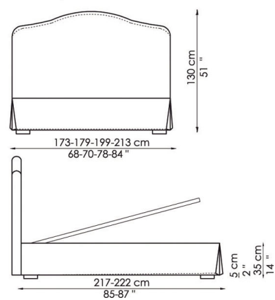
Lip contenitore with storage
