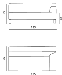
Yali - element 3-seater arm right
