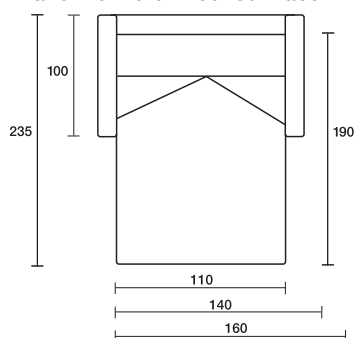
Piano letto / Bed surface
